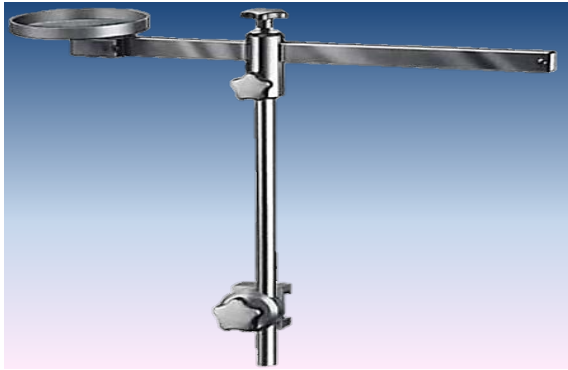
Figure 13: Adjustable supporting plate for laryngoscope holder
